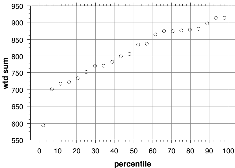
Percentiles Plot
