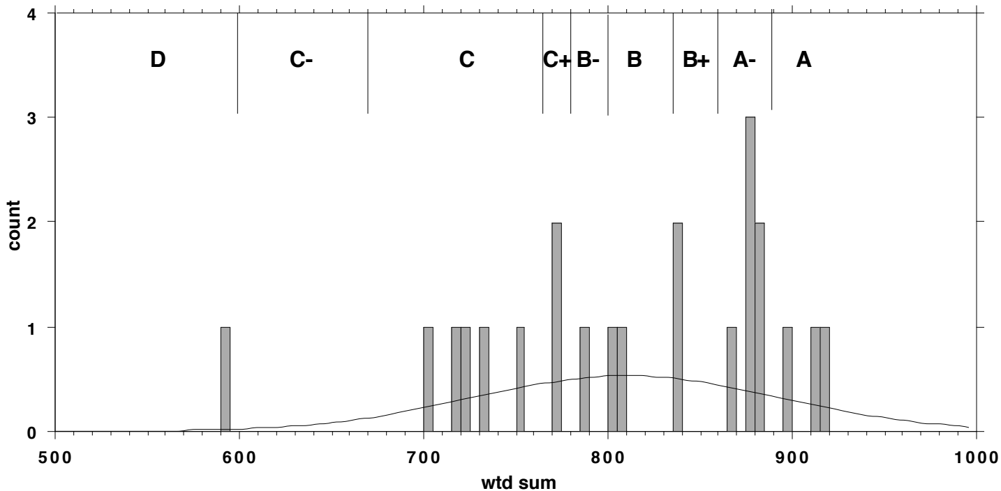
Histogram
