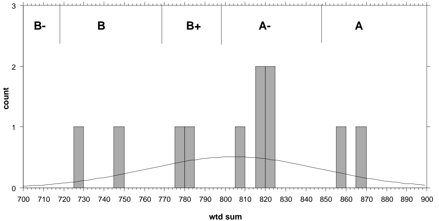
Histogram
