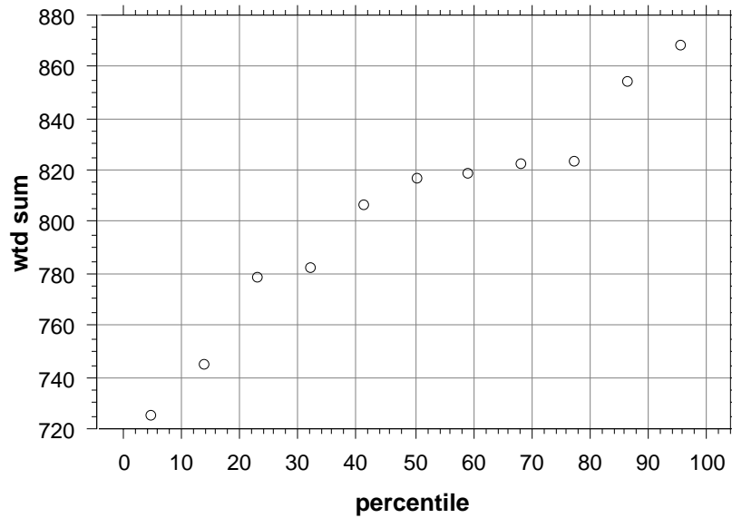
Percentiles Plot
