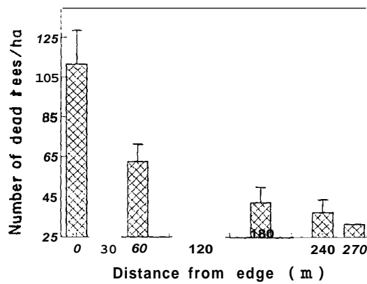
FIG. 6. Changes in numbers of standing dead trees (snags) and fallen boles (logs) with distance from the edge (0 m) into the interior forest. Data are means and 1 SE. N = 14. Data at 270 m are from Franklin and DeBell (1988) and Franklin et al. (1981).
