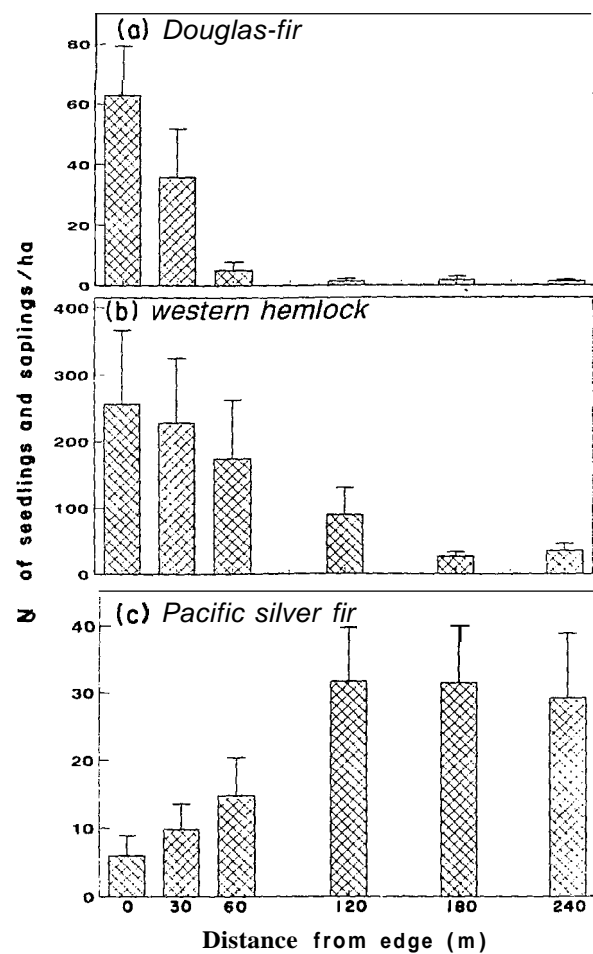
FIG. 7. Numbers of (a) Douglas-fir, (b) western hemlock, and (c) Pacific silver fir seedlings (≤ 100 cm) and saplings (10–200 cm), with distance from the edge (0 m) into the interior forest. Data are means and 1 SE. N = 15.
