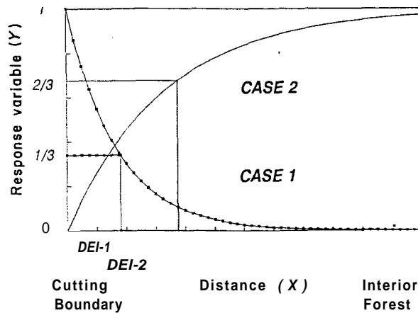
FIG. 2. Depth-of-edge influence (DEI) for two example cases: DEI calculated as Y = Y_0 + (2/3)(Y_0 - Y_{240}) and as Y = Y_0 - (2/3)(Y_0 - Y_{240}) , where Y is the response of a given biological variable from an edge (0 m, Y_0 ) into the forest (240 m, Y_{240} ).
