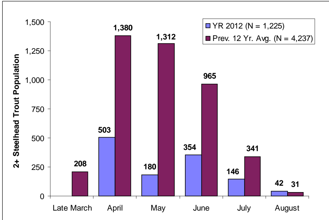
Figure 9. Comparison of 2+ steelhead trout population emigration by month in YR 2012 with the previous twelve year average, upper Redwood Creek, Humboldt County, CA. Numeric values above columns represent number of individuals.
