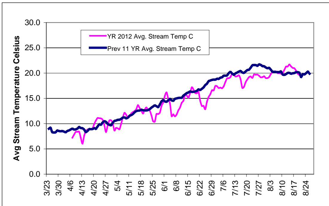
Figure 11. Comparison of average daily stream temperature in YR 2012 with the previous eleven year average, upper Redwood Creek, Humboldt County, CA.
