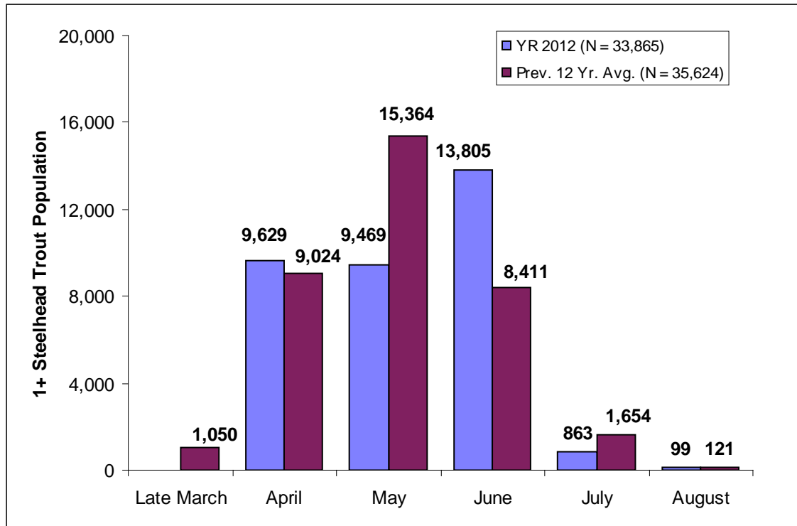
Figure 7. Comparison of 1+ steelhead trout population emigration by month in YR 2012 with the previous twelve year average, upper Redwood Creek, Humboldt County, CA. Numeric values above columns represent number of individuals.
