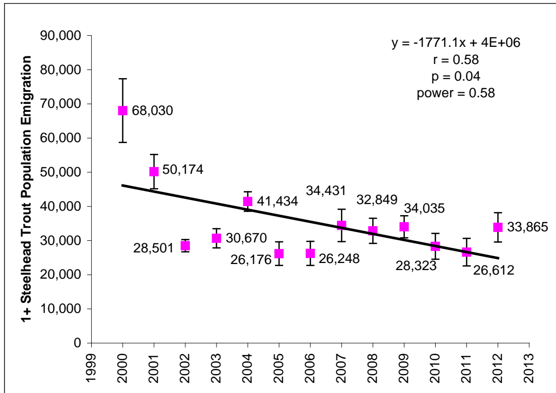
Figure 6. 1+ steelhead trout population estimates (error bars are 95% confidence interval) in thirteen consecutive years. Numeric values next to box represent number of individuals. Line of best fit is a regression line, with corresponding equation, correlation value (r), p value, and power of the statistical test.
