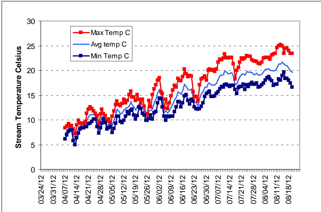
Figure 10. Average, minimum, and maximum stream temperature (Celsius) at the trap site (Rm 33), upper Redwood Creek, Humboldt County, CA., 2012.
